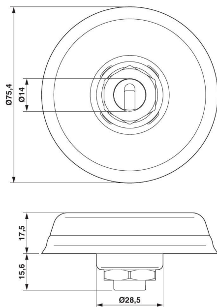
Figure 10 Dimensions
